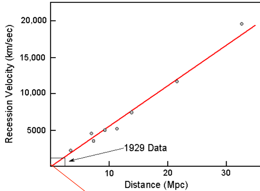
Hubble & Humason (1931)
